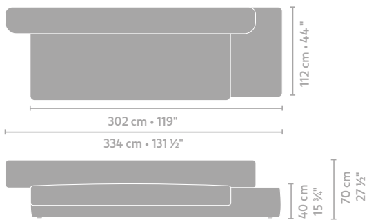
central/terminal element with plateau L/R 302 x 112 metrage 15,84
