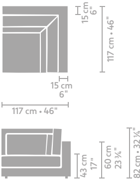
corner L/R deep 10,12
