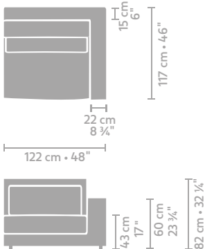
element 122 x 117 arm L/R deep 8,42
