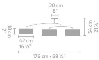
suspension 3 176 x 54
