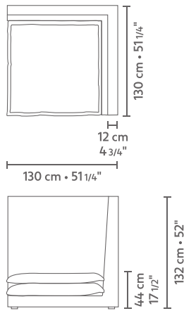
corner high 130 x 130 L/R * metrage (m) on request
