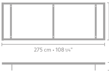
frame 275 x 100
