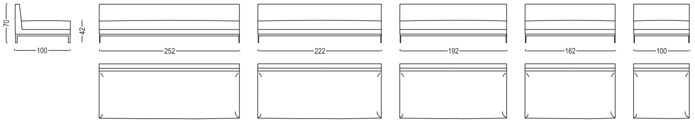
4 seater - 0 arm
